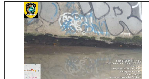
Abutment scouring
